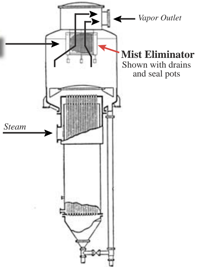
Rising Film Evaporator
