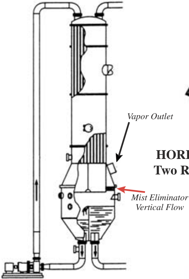
Falling Film Evaporator
